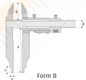
Monoblock Nonius 1/20 = 0,05 mm + 1/128 inch
