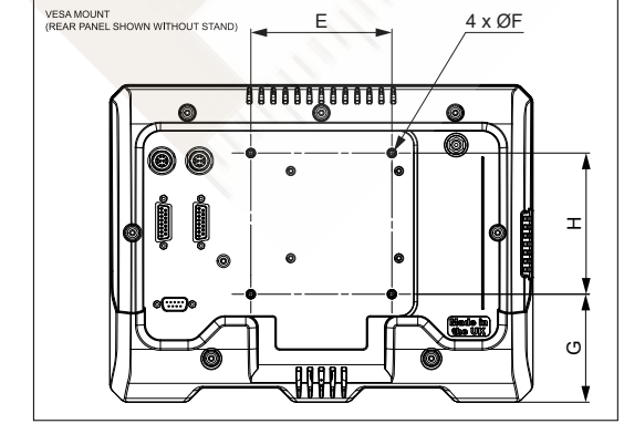
T-Box™ 2 back panel allows for 2 transducers to connect simultaneously, 1 RS-232 serial port and 2 ancillary ports
